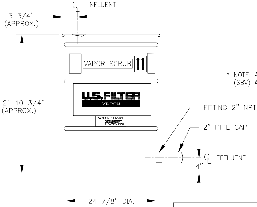
PLAN VIEW
