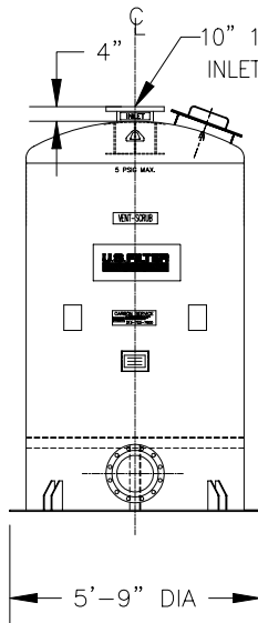
ELEVATION VIEW
